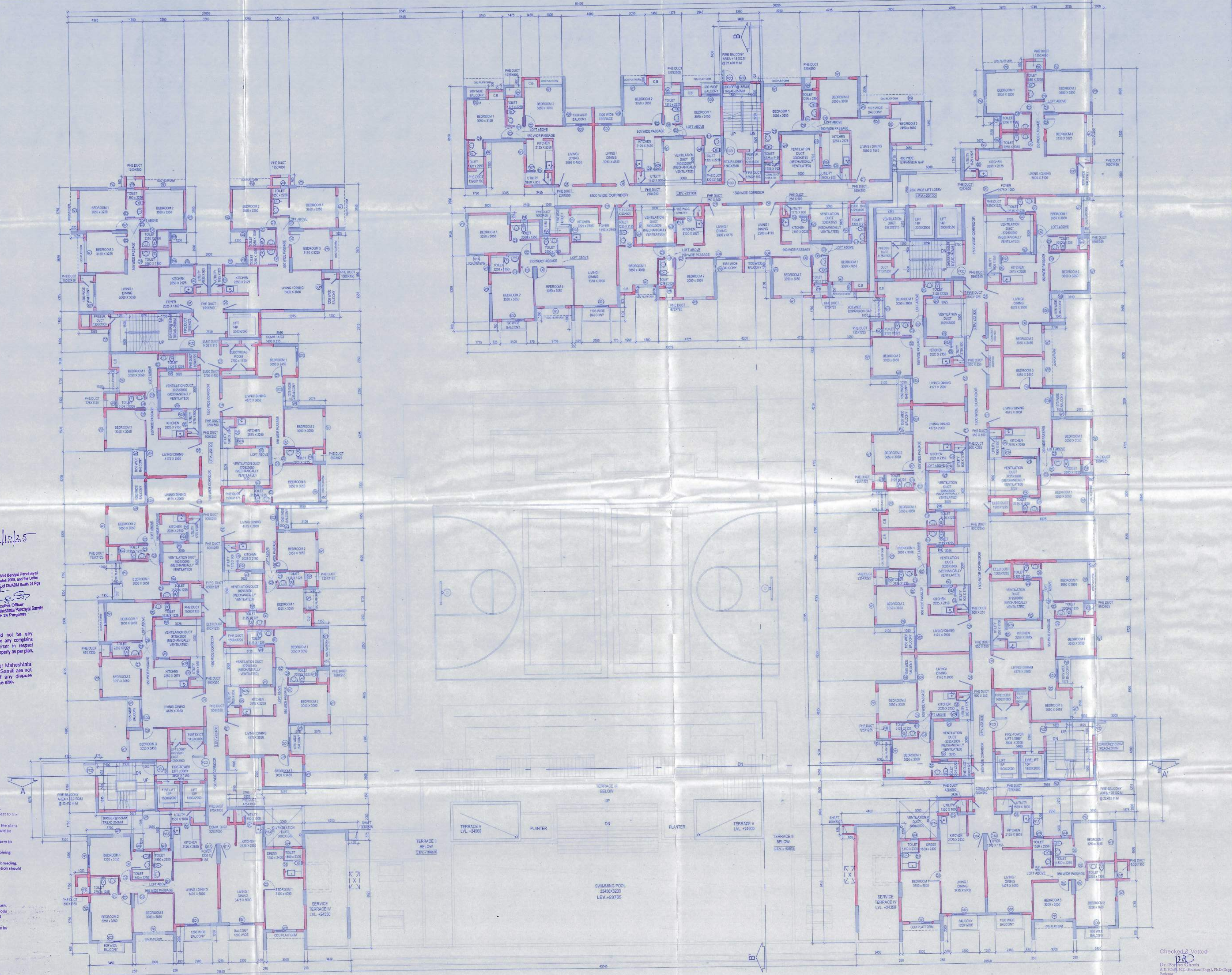
7TH FLOOR PLAN LVL 23.100 M
